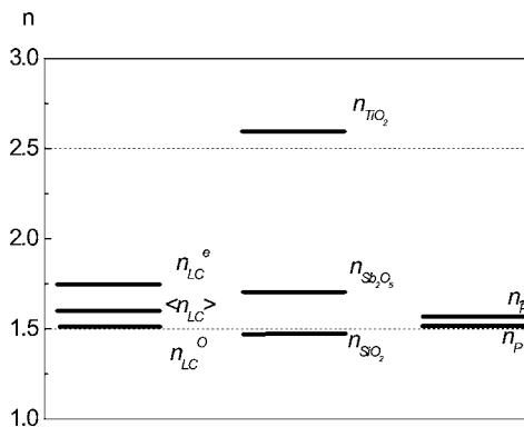
FIG. 5. The refractive index diagram for the components of the studied composites.
