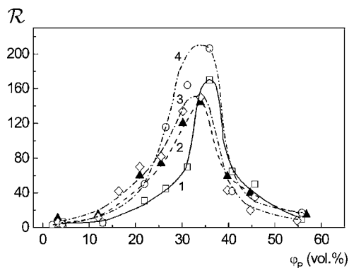
FIG. 7. \mathcal{R} vs polymer concentration curves for E7-MNP-polymer composites. 1, \phi_{MNP} = 0 vol %; 2, \phi_{Sb_2O_5} = 1 vol %; 3, \phi_{SiO_2} = 1 vol %; 4, \phi_{TiO_2} = 0.5 vol % (powder). The concentrations of MNP are optimized for maximal contrast and sample uniformity. The lines are just for guidance.
