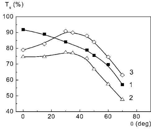
FIG. 10. The sample transmittance ( T_s ) vs. incidence angle curves for polymer stabilized E7-MNP samples. 1-E7-SiO 2 ( \varphi_{\text{SiO}_2} = 0.5 vol. %), 2-E7-TiO 2 ( \varphi_{\text{TiO}_2} = 0.5 vol. %), 3-E7-Sb 2 O 5 ( \varphi_{\text{Sb}_2\text{O}_5} = 0.5 vol. %). For all samples \varphi_P = 5 vol. %. The lines are just for guidance.
