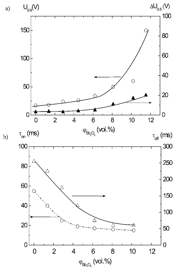
FIG. 6. U_{0.9}, \Delta U_{0.5} (a) and \tau_{on}, \tau_{off} (b) as functions of MNP concentration for polymer stabilized E7-Sb 2 O 5 composites ( \phi_P = 5 vol %). The lines are guides for the eye.
