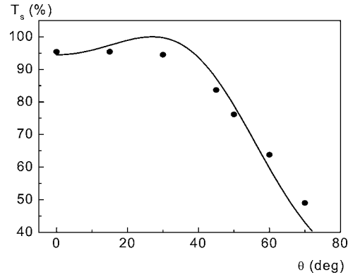
FIG. 11. Transmittance as a function of incidence angle \theta for the pure PDLC sample with \varphi_{LC} = 63 vol % and \varphi_{MNP} = 0. Points correspond to experimental data, solid line represents the theoretical curve computed from Eqs. (7)–(10) at \varphi_d = 0.44, \theta_m = 27°, and R_d = 0.35 \mu\text{m} . The bipolar order parameter S_d and the effective refractive index n_m are estimated at 0.7 and 1.5569, respectively.
