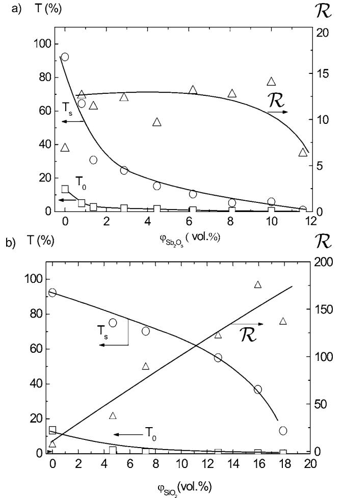
FIG. 3. T_0 , T_s , and \mathcal{R} vs \varphi_{MNP} curves for polymer stabilized E7-Sb 2 O 5 (a) and E7-SiO 2 (b) composites. Polymer concentration is 5 vol %. The lines are just a guide for the eye.
