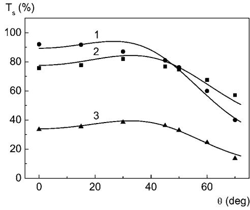
FIG. 12. Transmittance T_s as a function of incidence angle \theta for LC-P-MNP samples of PDLC morphology ( \varphi_{LC}=63 vol %). Points represent experimental data obtained for the samples (1) PDLC doped with \text{SiO}_2 MNPs, \varphi_{MNP}=1.3 vol %; (2) PDLC doped with \text{Sb}_2\text{O}_5 MNPs, \varphi_{MNP}=1.3 vol %; (3) PDLC doped with \text{Sb}_2\text{O}_5 MNPs, \varphi_{MNP}=3.3 vol %. Solid lines 1–3 represent the theoretical curves computed from Eqs. (7)–(10) at the following values of the fitting parameters: (1) \theta_m=27^\circ , n_m=1.5545 , \varphi_{MNP}=0.013 , R_{MNP}=0.2 \mu\text{m} ; R_d=0.3 \mu\text{m} ; (2) \theta_m=34^\circ , n_m=1.5578 , \varphi_{MNP}=0.013 , R_{MNP}=0.2 \mu\text{m} ; R_d=0.2 \mu\text{m} ; (3) \theta_m=36^\circ , n_m=1.561 , \varphi_{MNP}=0.033 , R_{MNP}=0.4 \mu\text{m} ; R_d=0.4 \mu\text{m} .
