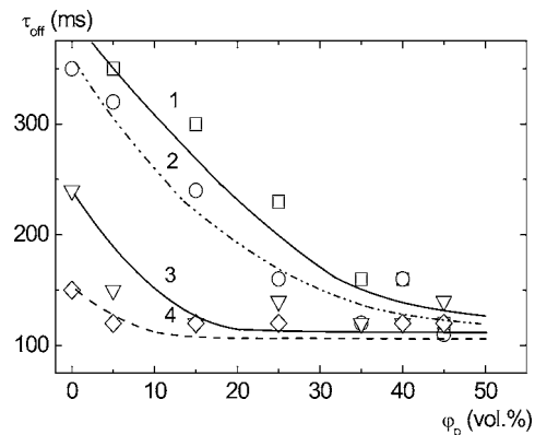
FIG. 9. \tau_{off} vs \phi_P curves for E7-P composites, nonfilled and filled with Sb 2 O 5 MNP. 1, \phi_{Sb_2O_5} = 0 vol %; 2, \phi_{Sb_2O_5} = 2.5 vol %; 3, \phi_{Sb_2O_5} = 4 vol %; 4, \phi_{Sb_2O_5} = 5 vol %. The lines are guides for the eye.
