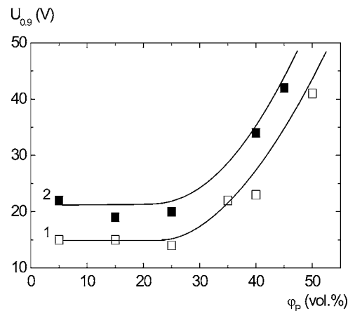
FIG. 8. U_{0.9} vs \phi_P curves for E7-P composites, nonfilled (1) and filled with Sb 2 O 5 MNP, \phi_{Sb_2O_5} = 5 vol % (2). The lines are guides for the eye.
