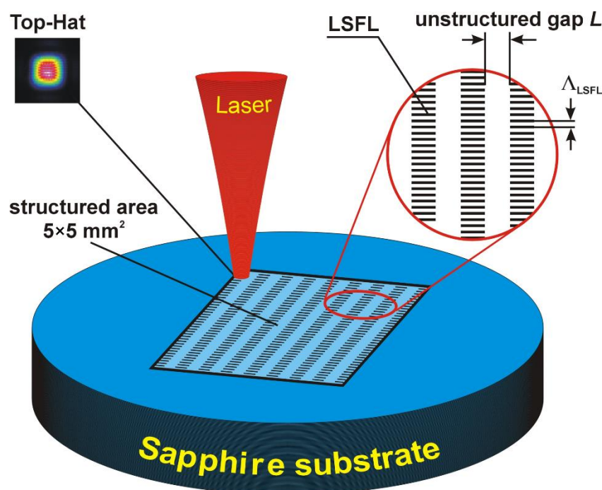
Figure 1. Schematic illustration of the sapphire structuring process. The structured area with a dimension of 5 \times 5\text{ mm}^2 has alternating high-quality structured lines (1D-LSFL), with a period \Lambda = 980\text{ nm} and depth A = 100\text{ nm} , and unstructured gaps, having a width, L , changing within 7\text{--}17\text{ }\mu\text{m} .
