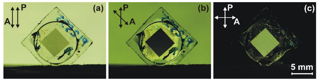
Figure 7. Photographs of the twist LC cell placed between a pair of polarizers with different angles of planes of polarization: (a) parallel, (b) twist angle \varphi \approx 33.5 degrees, and (c) perpendicular. The LC cell consists of the reference (rubbed PI2555 layer) and tested substrate, having the structured sapphire surface with 1D-LSFL (23 \mu\text{m} width) and unstructured gaps (11 \mu\text{m} width). The twist angle, \varphi^\Sigma , of the processed area of the LC cell is about 33.5 degrees. The thickness of the twisted LC cell is d = 24.6 \mu\text{m} . The rubbing direction of the reference substrate (PI2555 layer) coincides with the plane of polarization of the polarizer, while the analyzer can rotate freely.
