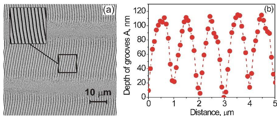
Figure 2. (a) SEM image of the sapphire surface with alternating both the high-quality 1D-LSFL with 23\text{ }\mu\text{m} and the unstructured gap with 7\text{ }\mu\text{m} widths. The portion of the structured line with area 10 \times 10\text{ }\mu\text{m}^2 is on an enlarged scale. (b) The cross-section of the 1D-LSFL taken with the AFM reveals an average value of the spatial period \Lambda of 980\text{ nm} and a depth, A , of 100\text{ nm} .
