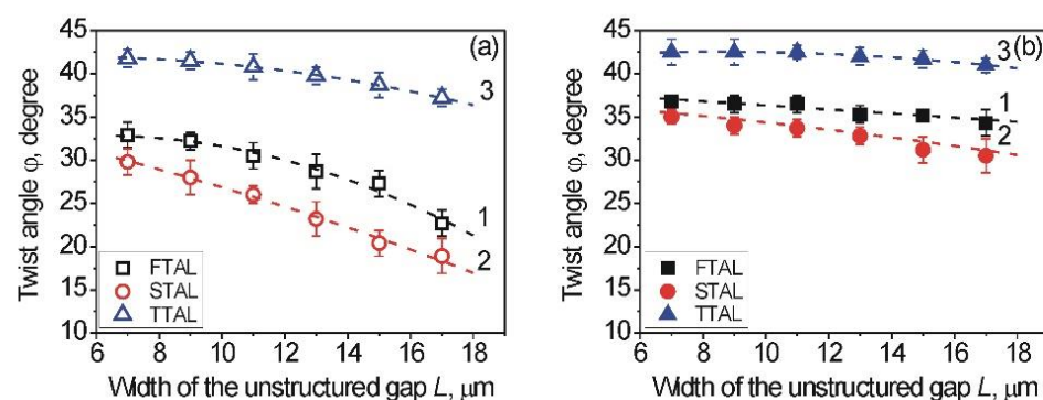
Figure 3. Dependence of the twist angle, \varphi , on the width, L , of the unstructured sapphire gaps in case of the FTAL (curves 1, black squares), STAL (curves 2, red circles), and TTAL (curves 3, blue triangles) for: (a) unstructured sapphire gaps, located between two 1D-LSFL (opened symbols) and (b) 1D-LSFL located nearby the unstructured sapphire gap (solid symbols). Data are average values of the twist angles, \varphi , measured at three different places of certain LC cells and for the three various samples, consisting of sapphire substrates possessing a certain width, L , of unstructured gaps. Error bars are absolute deviations of the twist angle from average values. The dashed curve is a guide to the eye.
