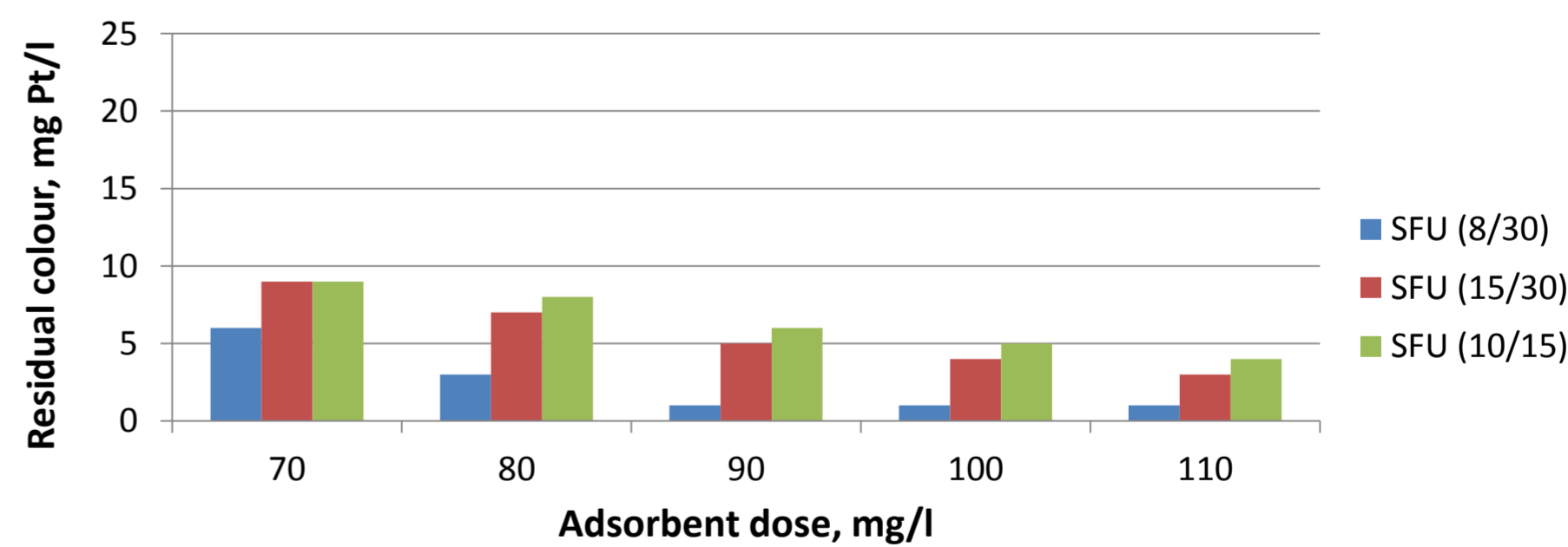
Figure 3. Humates adsorption.
