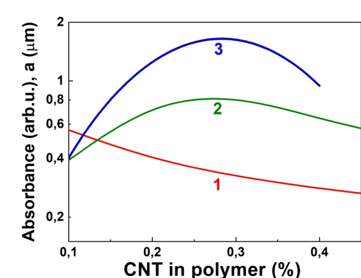
Fig. 6. Dependences on CNTs content of: (1) average distance a between CNT, (2) geometric approximation - characteristic volume around CNT; (3) experimental dependence from Fig. 4b.
