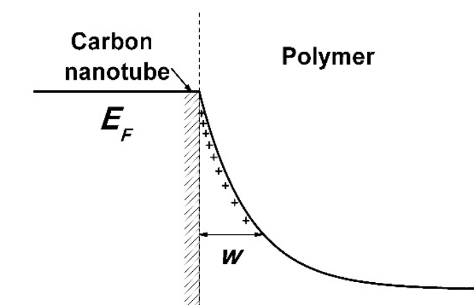
Fig. 7. Band bending and SCR width w at the “polymer-CNTs” boundary.
