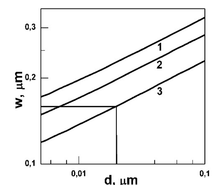
Fig. 8. Dependence of SCR width w around cylindrical nanotubes on its diameter for surface potential Y_s : 1-12 kT ; 2-8 kT ; 3-4 kT .
