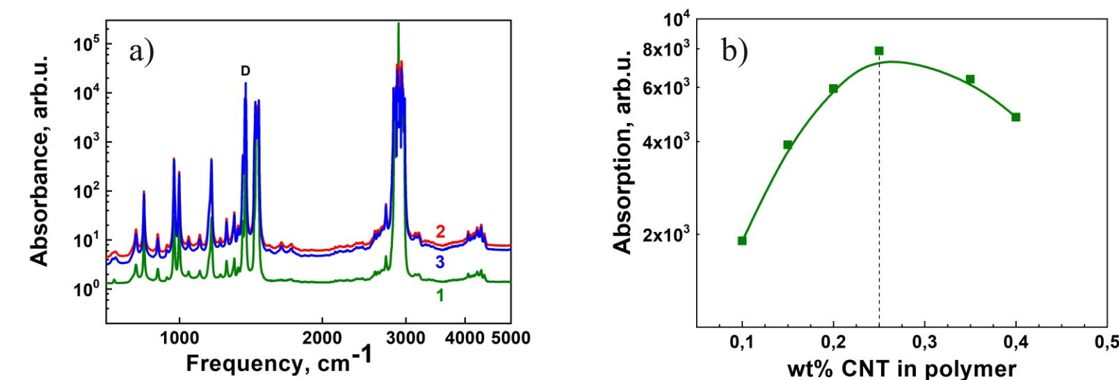
Fig. 4: a - IR absorption spectra of polypropylene (curve 1), composite “polypropylene-carbon nanotubes” (curve 2) and the ratio of curves 1 and 2 (curve 3); b - IR absorption by sp^3 hybridization bonds (D) in composites based on polypropylene vs the carbon nanotube content in polymer.
