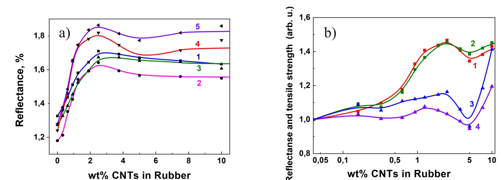
Fig. 5: a - IR reflectance maxima of composite “rubber-carbon nanotube” vs the carbon nanotube content in polymer in the area of CH deformation vibrations (1, 2 and 3) and valence vibrations (4, CH 3 and 5, CH 2 ); b - Relative IR reflectance R/R_0 in the area of CH 3 (curve 1) and CH 2 (curve 2) valence vibrations and the relative tensile strength N/N_0 for two types of composites “polybutadien rubber-carbon nanotube” (curves 3-4) vs the carbon nanotube content in rubber.
