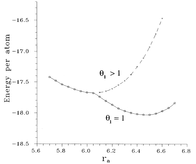
FIG. 8. The energies of the GS \theta_1 = 1 configuration (full curve) and the metastable \theta_1 = 17/16 configuration (broken curve) as functions of r_a . \theta = 17/16 , \varepsilon_a = 6 , \beta = 1.9 , and \beta' = 0.19 .
