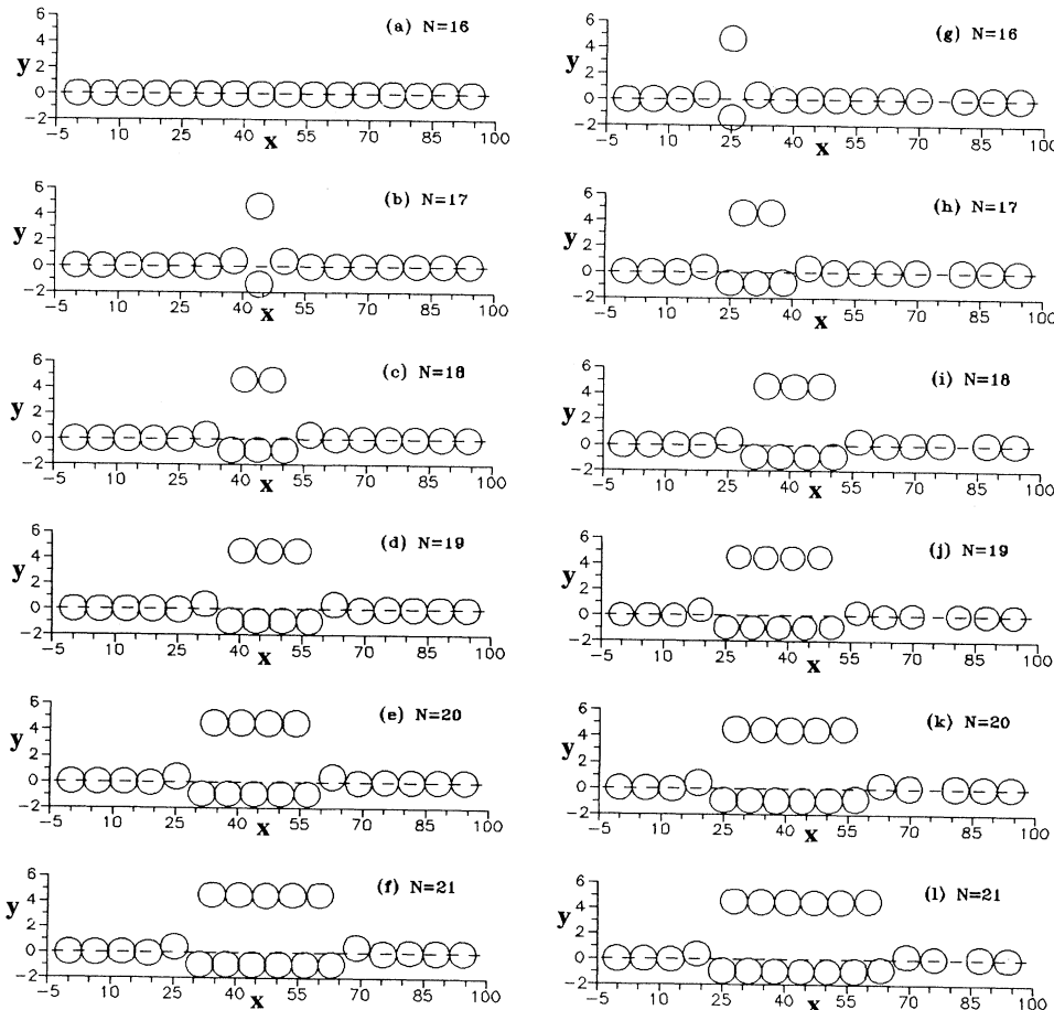
FIG. 4. Atomic configurations for the model with the generalized-Morse interaction (8). M = 16 , r_a = 7 , \varepsilon_a = 6 , \beta = 1.9 , and \beta' = 0.19 . The number of substrate potential minima is M = 16 , the coverage is \theta = N/M and is increased by increasing the number N of adatoms from 16 to 21. In this range of coverage, for each N , the system has two stable configurations: the first ones (a-f) are obtained with a full coverage of 16 atoms in the first layer, while the second class of configurations (g-l) has only 15 atoms in the first layer.
